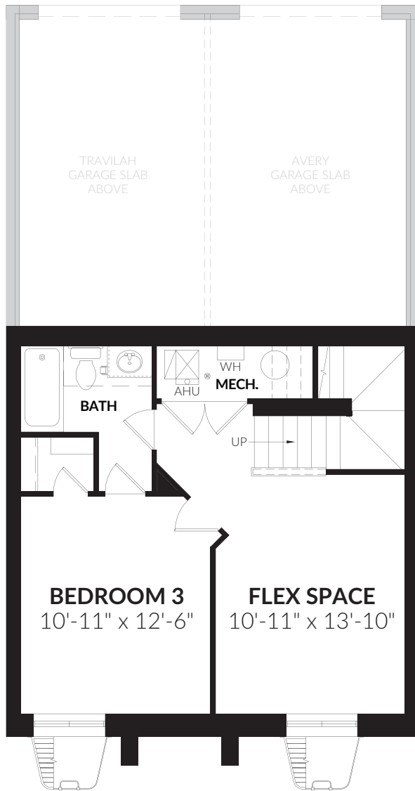
BASEMENT PLAN SHOWN WITH ELEVATION 1
