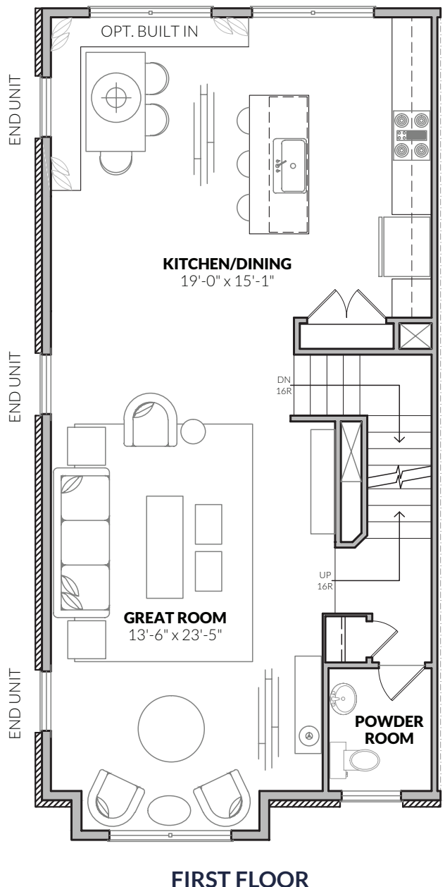
OPT. FIRST FLOOR WITH ALTERNATE KITCHEN
