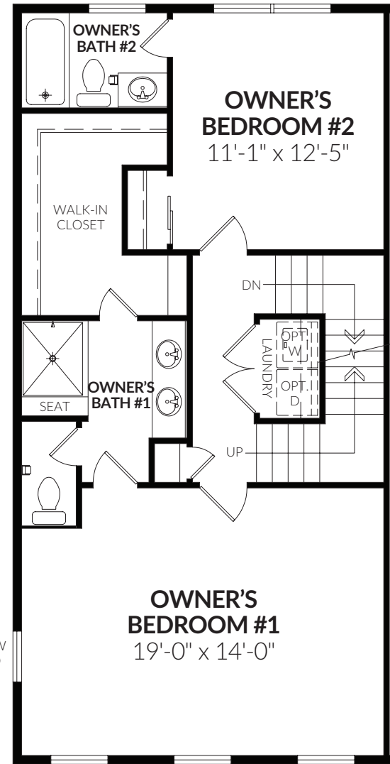
OPT. ALTERNATE SECOND FLOOR SHOWN WITH STAIRS TO OPT. LEFT
