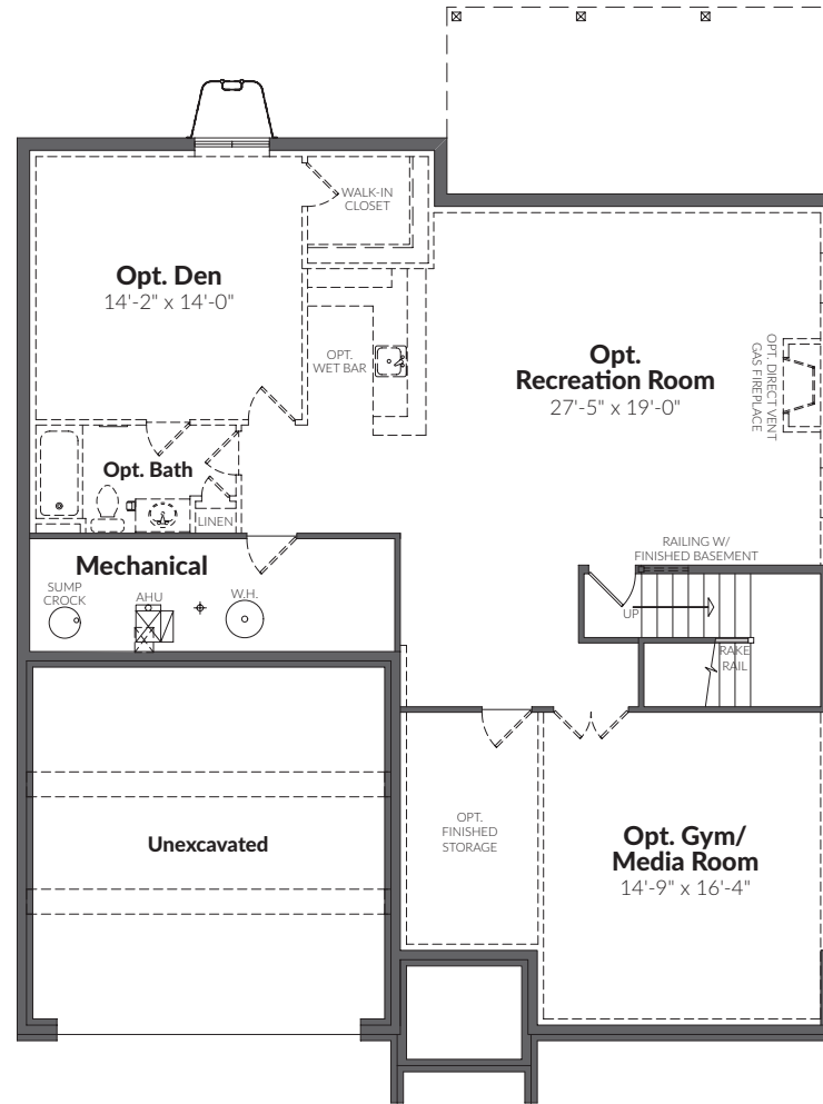
BASEMENT FLOOR PLAN SHOWN WITH ELEVATION 1 & OPT. EXTENSION (INCLUDED)
