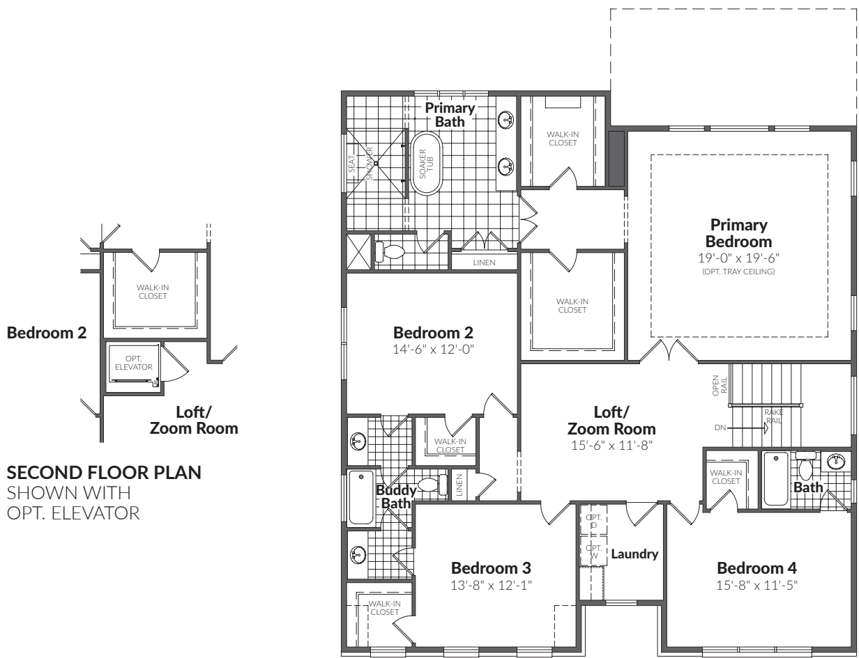
SECOND FLOOR PLAN SHOWN WITH ELEVATION 1 & OPT. EXTENSION (INCLUDED)
