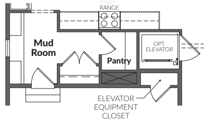
FIRST FLOOR PLAN SHOWN WITH OPT. ELEVATOR
