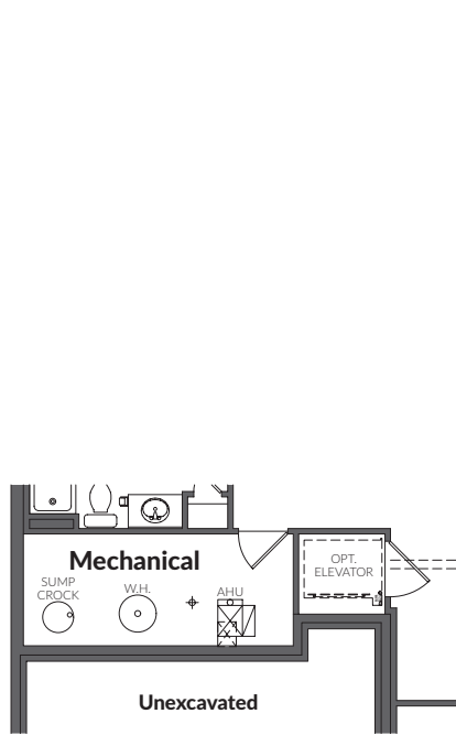
BASEMENT FLOOR PLAN SHOWN WITH OPT. ELEVATOR
