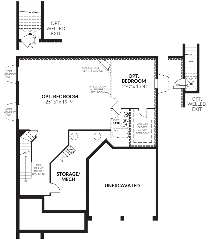
LOWER LEVEL
